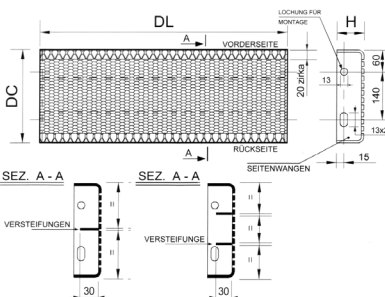
SUPER FELDKIRCH DEBELINA 3 mm
